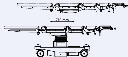
Longitudinal slide adjustment
